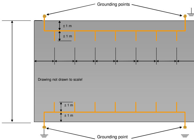
Picture 3 – Copper strip layout for rooms > 50 m^2 , alternative B
